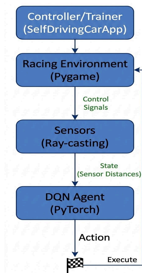
Figure: The architecture separates the learning components from rendering, allowing the same trained model to run in both headless training and live Pygame evaluation without changing the main learning code.
